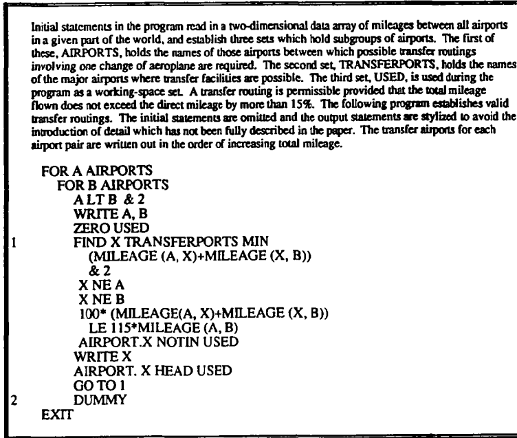
Figure 7. Problem Statement and Example of CSL Code [Buxton 1962, p. 199]
