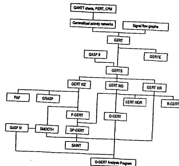
Figure 14. The GERT Family Tree (from [Pritsker 1990, p. 243])
