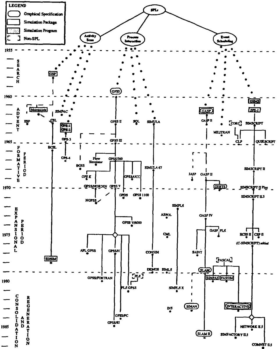
Figure 1. The Genealogical Tree for Simulation Programming Languages
