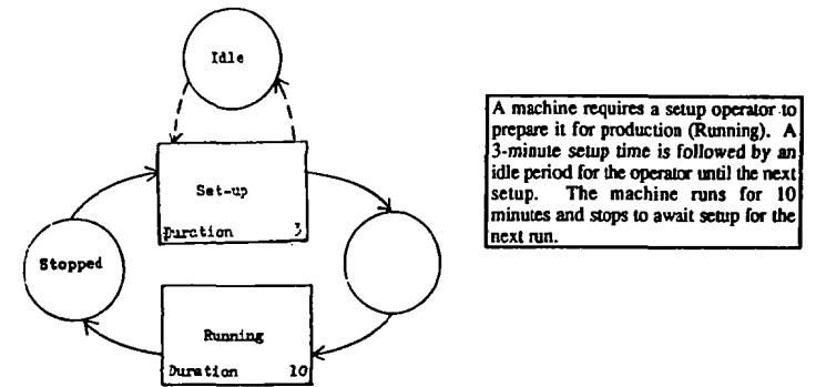
(b) The Activity Cycle Example (from [ECSL-CAPS Reference Manual 1978, p. 9])
