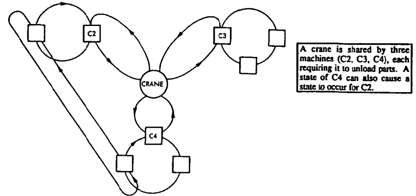
(a) The Wheel Chart Example (from [Tocher 1966, p. 129])
